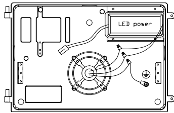
Wire Connection
