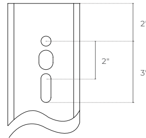
DRILL PATTERN (TOP OF POLE)
