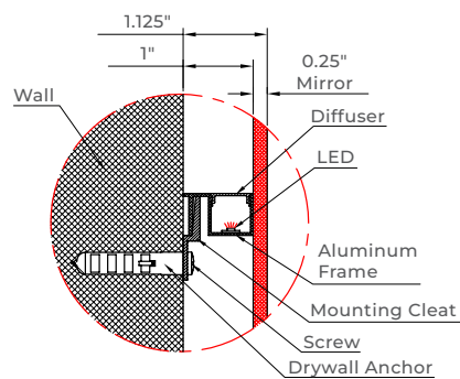
FIGURE A: MIRROR CROSS SECTION
