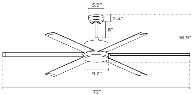
MESOS-72 WITH LIGHT KIT
