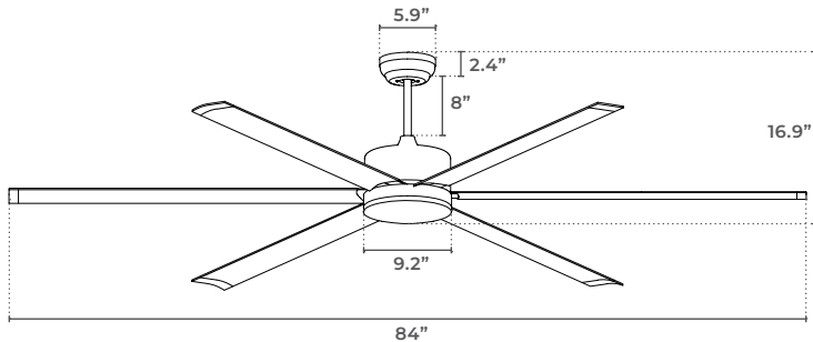
MESOS-84 WITH LIGHT KIT
