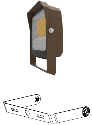
YOKE MOUNT
