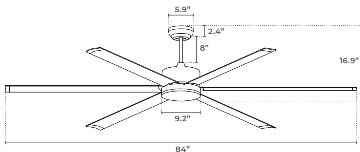
MESOS-84 WITH LIGHT KIT
