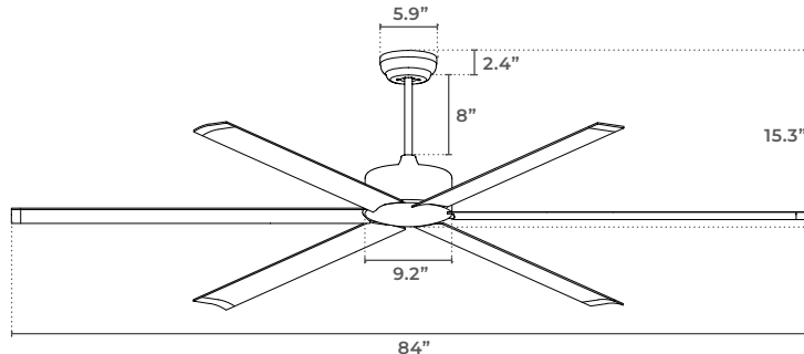
MESOS-84 WITHOUT LIGHT KIT
