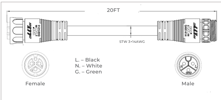
STAR-20JC 20' Jumper Cable
