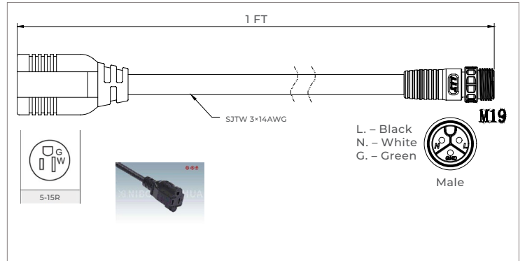
STAR-PA Plug Adapter, LLT 3P F to NEMA 5-15P Adapter
