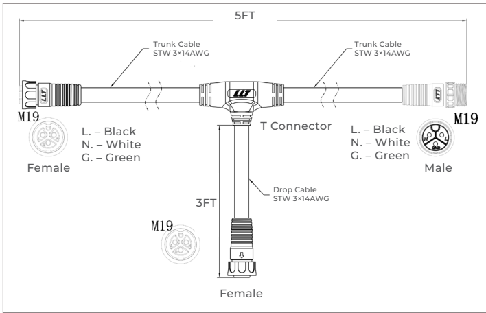
STAR-TC 5' Trunk Cable
