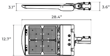
Slip Fitter
