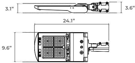
Slip Fitter
