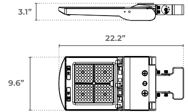
Yoke Bracket
