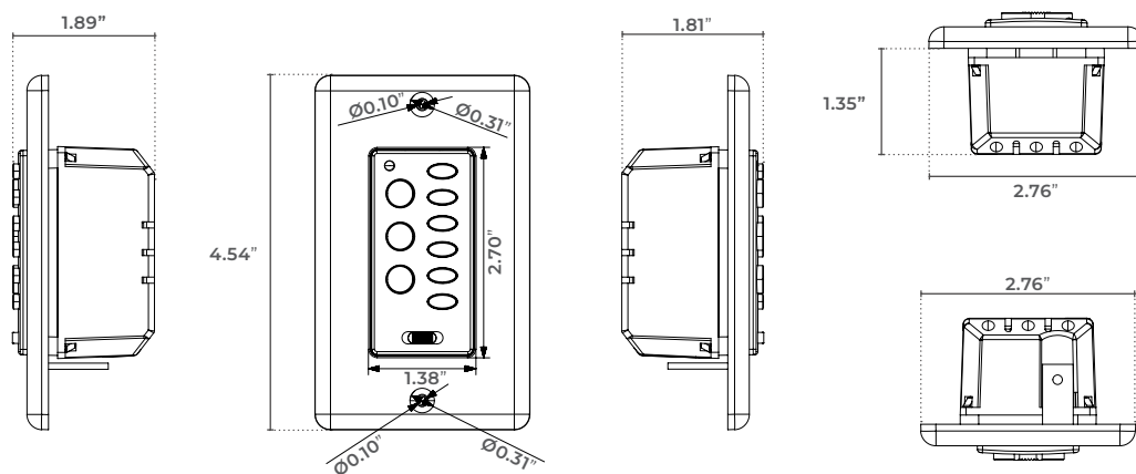
6WC-DIM DIMENSIONS
