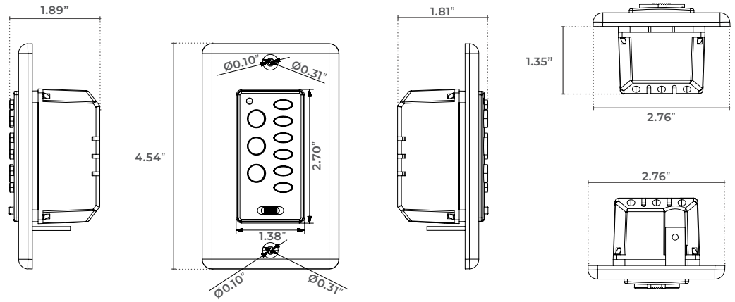
6WC-DIM DIMENSIONS
